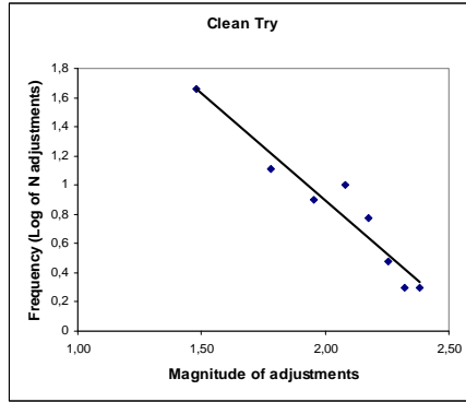
Figure 2.b Power law
