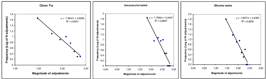
Figure 3. Power law distribution
